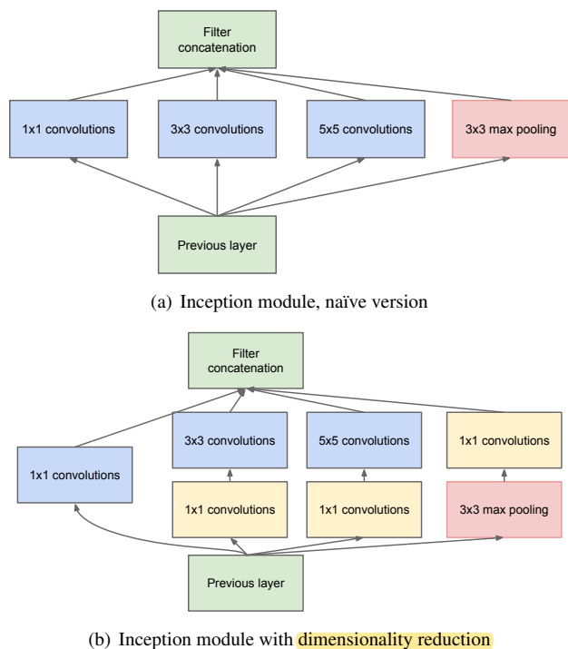
Figure 2: Inception module
